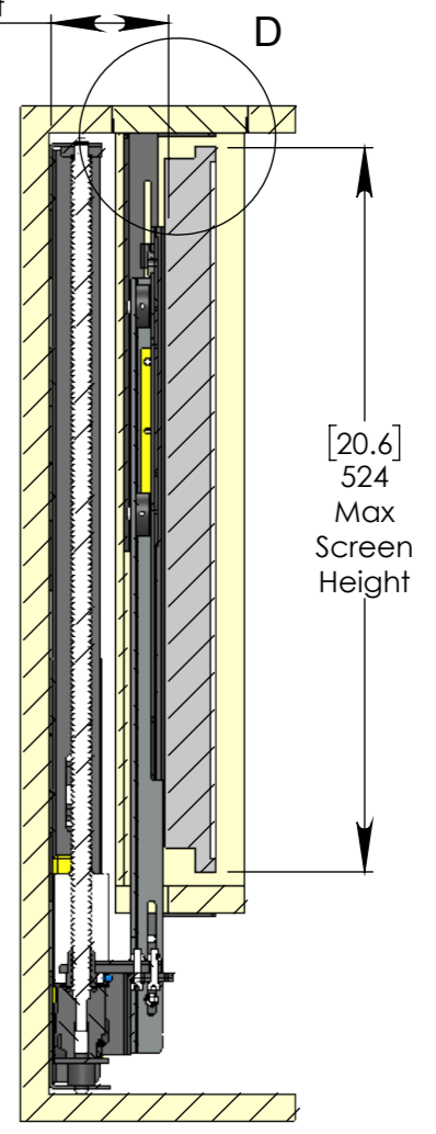
SECTION B-B
