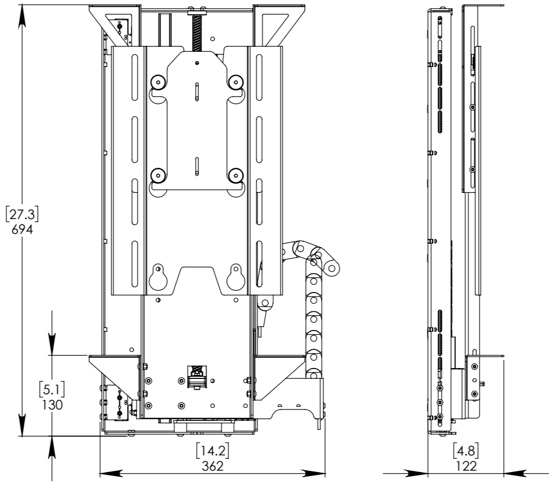
MECHANISM - DOWN POSITION
