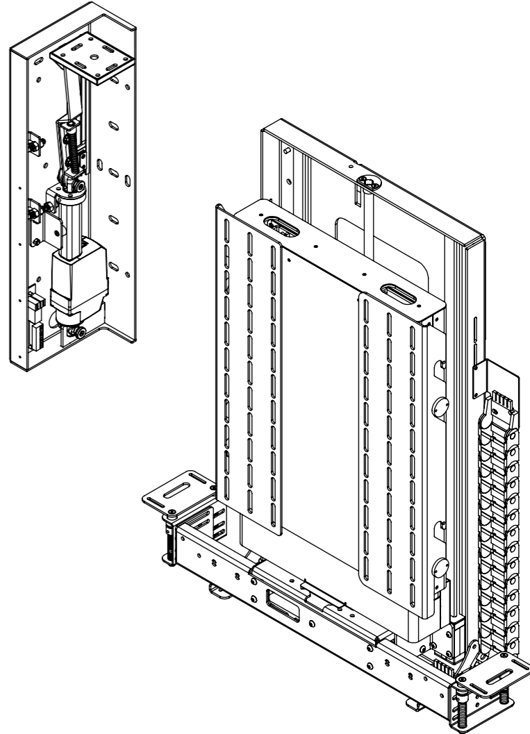
MECHANISM - DOWN POSITION
