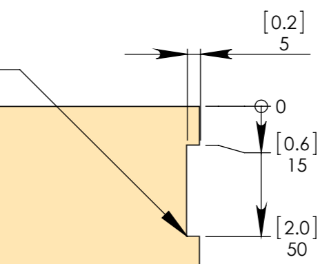
Cut-out for EFA Push Rod
